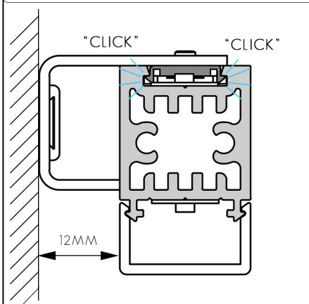
FIG. 2 - ENSURE EXTRUSION IS MOUNTED SECURELY
