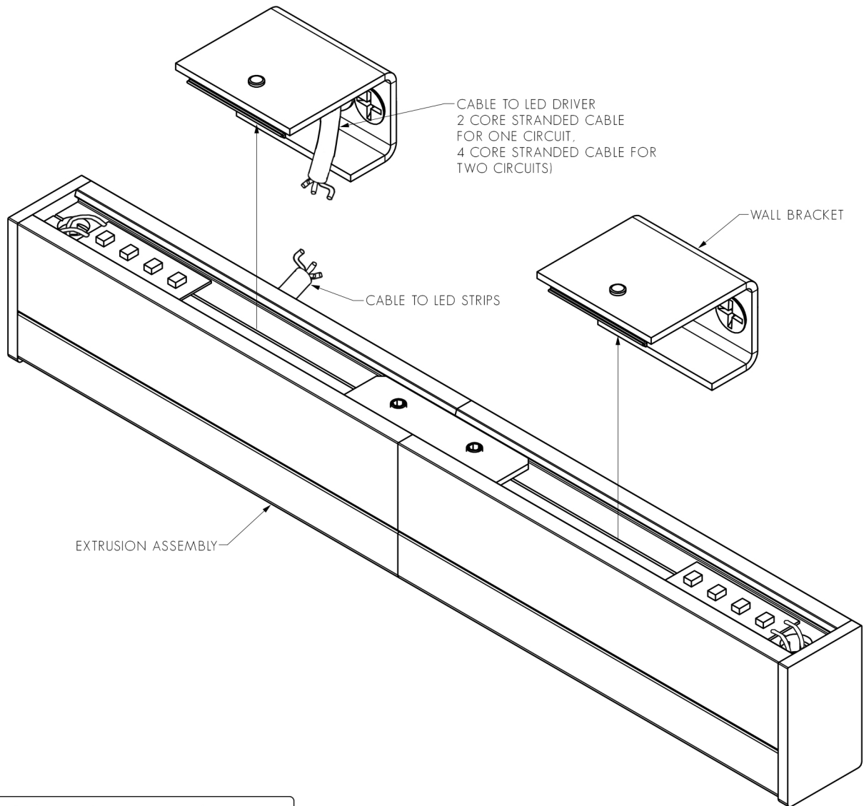
FIG. 2 - ENSURE EXTRUSION IS MOUNTED SECURELY
