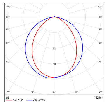
Polar curve for 600 lumen LED strip with opal diffuser.
