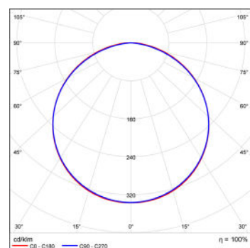
Polar curve for 2250 lumen LED strip with opal diffuser.
