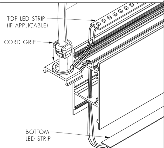
FIG. 2 - FASTEN CABLE USING CORD GRIP
